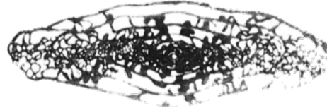
Triticites sp. F Nestell 1989
