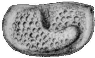
Kirkbyella typa Coryell & Booth 1933
